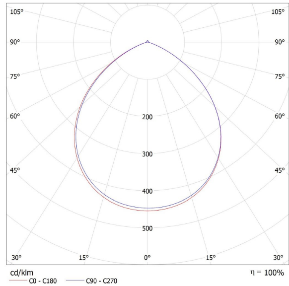
Polar curve
