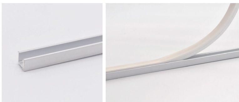
Aluminium profile 1000x9x6mm(L x W x H)
