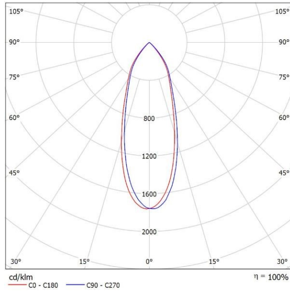
TUBELLO 8 - beam angle 40°
