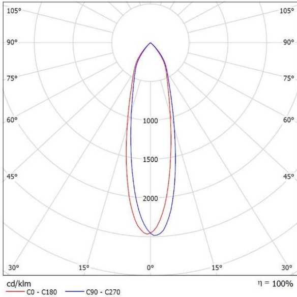
TUBELLO 8 - beam angle 25°
