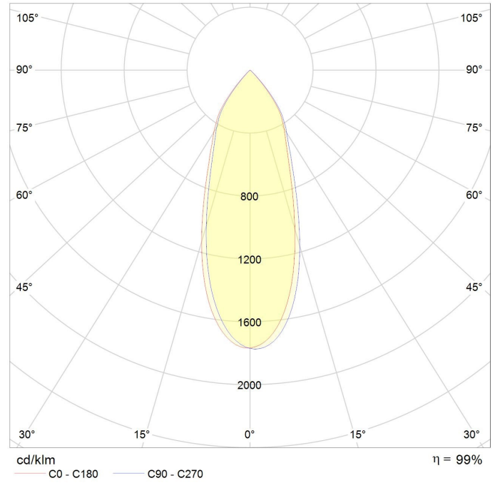
CEFE11 - beam angle 40°
